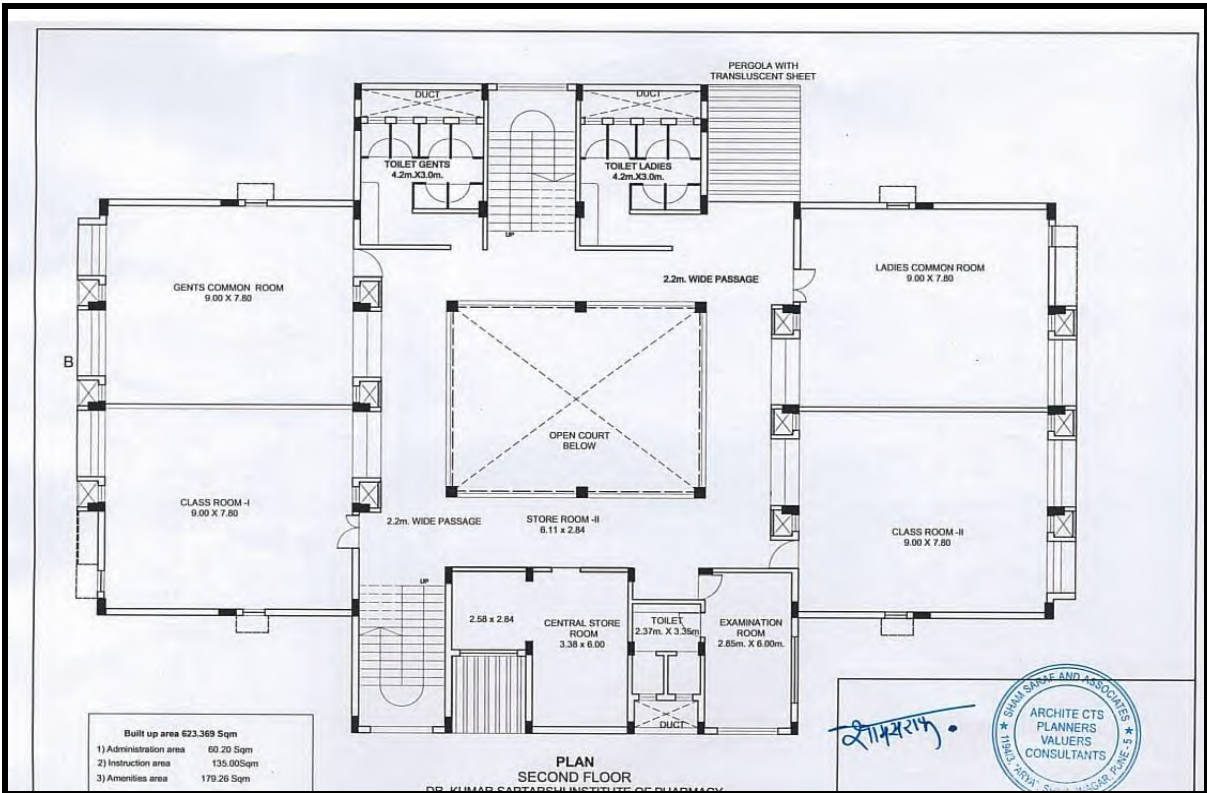
Second Floor
