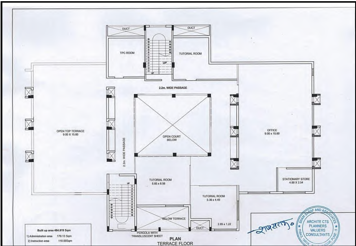
Terrace Floor
