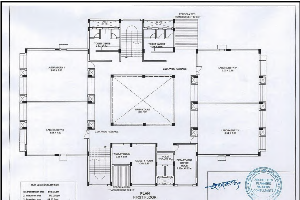
Frist Floor
